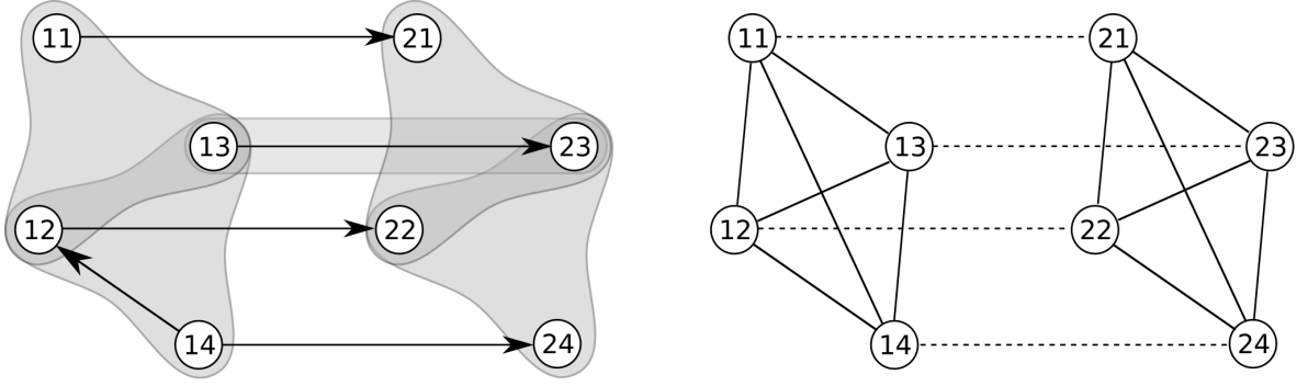
Figure 1: The prime hypergraph H (left-hand side) with arc set E(H) = \{e_1 = (\{11, 12, 13\}, \{12, 13, 14\}), KA : e_2 = (\{21, 22, 23\}, \{22, 23, 24\}), e_3 = (\{14\}, \{12\}), e_4 = (\{11\}, \{21\}), e_5 = (\{12\}, \{22\}), e_6 = (\{13, 23\}, \{13, 23\}), e_7 = (\{14\}, \{24\}), e_8 = (\{13\}, \{23\})\} admits a non-trivial prime factorization of its 2-section [H]_2 (right-hand side) into K_4 \square K_2 . The vertices of H are labeled w.r.t. its pre-coordination given by the coordinatization of [H]_2 . For the first arc e_4 of the lexicographic ordered arc set E_{\text{lex}} = \{e_4, e_1, e_5, e_8, e_6, e_3, e_7, e_2\} we can observe that the increment \text{inc}(e_4, 2) = (\{12\}, \{22\}) = e_5 \in E_{\text{lex}} . Analogously, \text{inc}(e_1, 1) = e_2 , \text{inc}(e_5, 2) = e_8 , and \text{inc}(e_8, 2) = e_7 are all contained in E_{\text{lex}} . However, when we arrive at the hyperedge e_6 we obtain that \text{inc}(e_6, 2) = (\{14, 24\}, \{14, 24\}) is not an arc of E_{\text{lex}} . Hence, applying Algorithm 1 would lead to an edge 12 in G_{\text{aux}} , resulting in a connected auxiliary graph and, H would be determined as prime. A second example for an arc e \in E_{\text{lex}} with \text{inc}(e, i) \notin E_{\text{lex}} is the edge e = e_7 .
